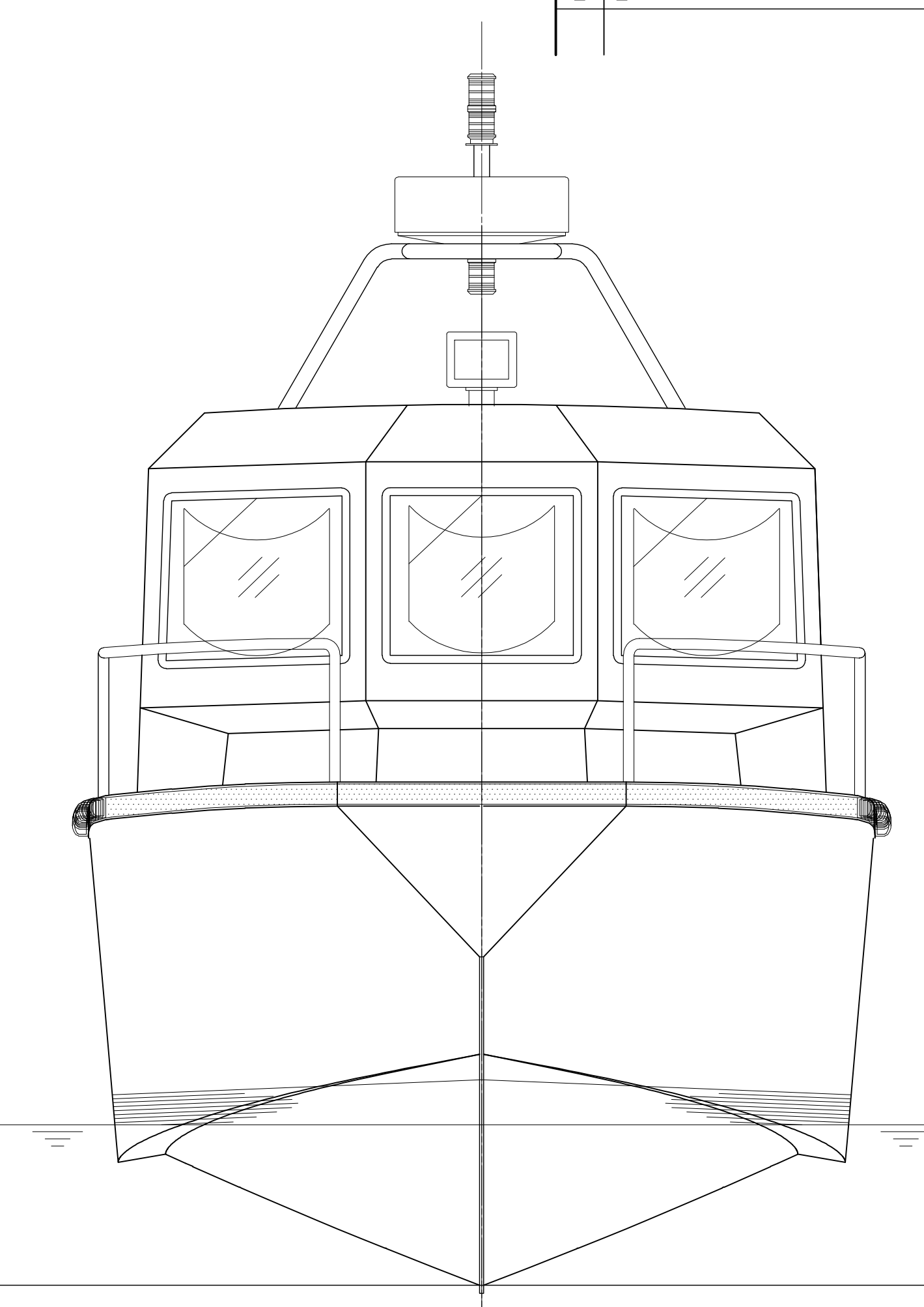
BOW VIEW
