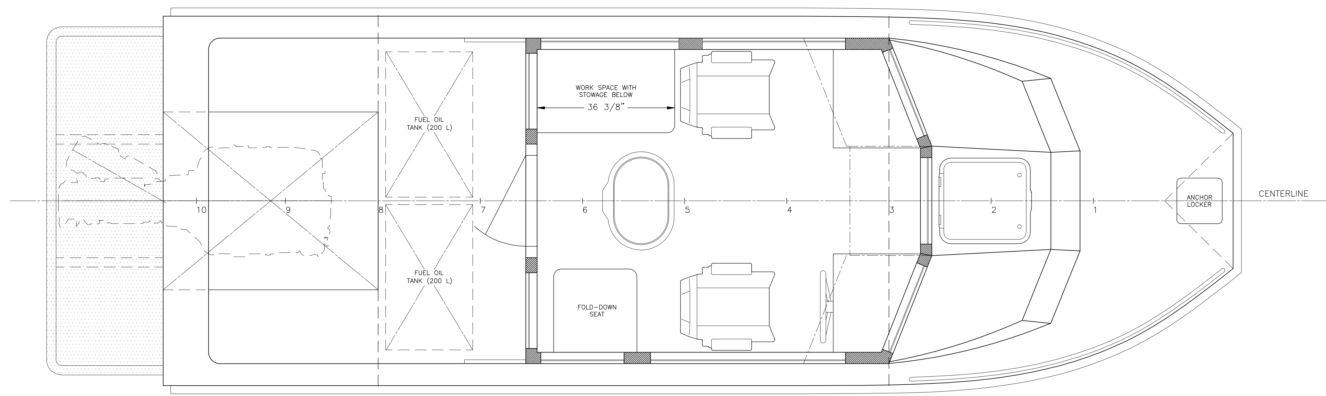
DECK PLAN
